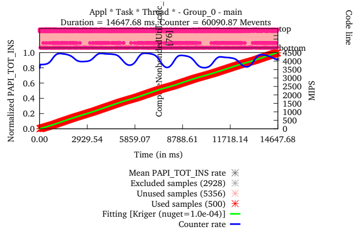
Figure 1.1: Evolution of graduated instructions for 444.namd.
